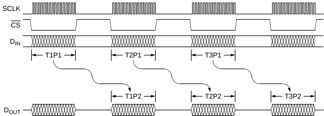
Figure 4-2 Single-Level Communications Queuing Detail
